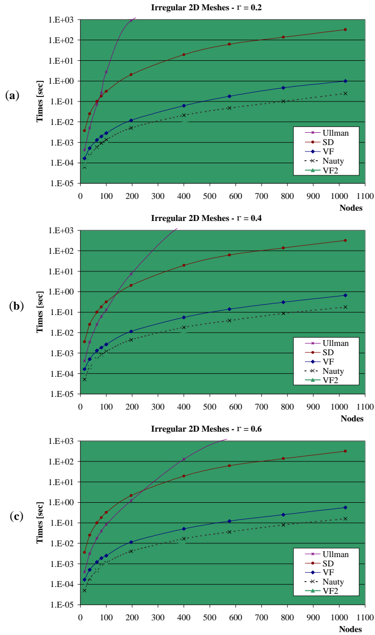
Fig. 3: The performance of the algorithms on Irregular 2D Meshes as a function of the graph size and for different values of \rho : (a) \rho = 0.2 , (b) \rho = 0.4 (c) \rho = 0.6 .
